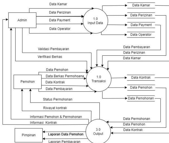
Gambar 4. Diagram overview / Diagram Level 0
